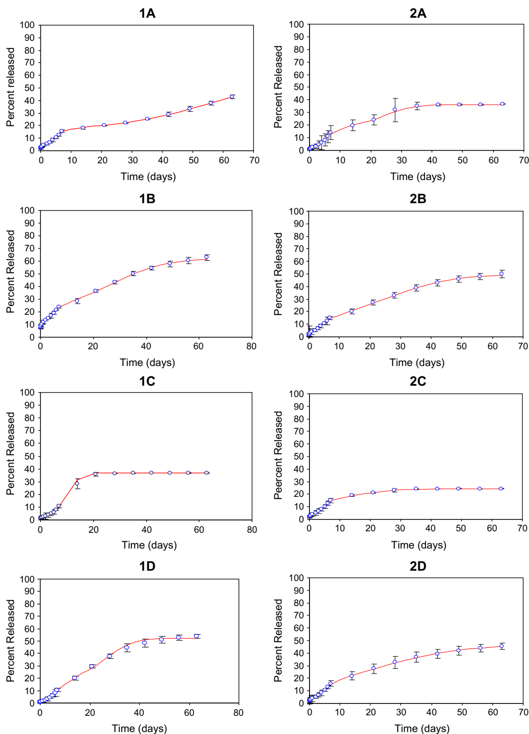
Fig. 4. Ciprofloxacin release from PLGA-excipt delivery systems. Open circles indicate the percent of ciprofloxacin released as a function of time (in days). The fitted line represents the ternary Gaussian model best-fit model. (Key: the terms a, b, c, and d refer to implants with constitution of PLGA90:10/ Span 85, PLGA 75:25/Tween 80, PLGA 65:35/Tween 80, and PLGA 50:50/PEG 300, respectively. Terms 1 and 2 refer to a lower and moderate level of drug loading as shown in Table 3.) (For interpretation of the references to colour in this figure legend, the reader is referred to the web version of this article.)
